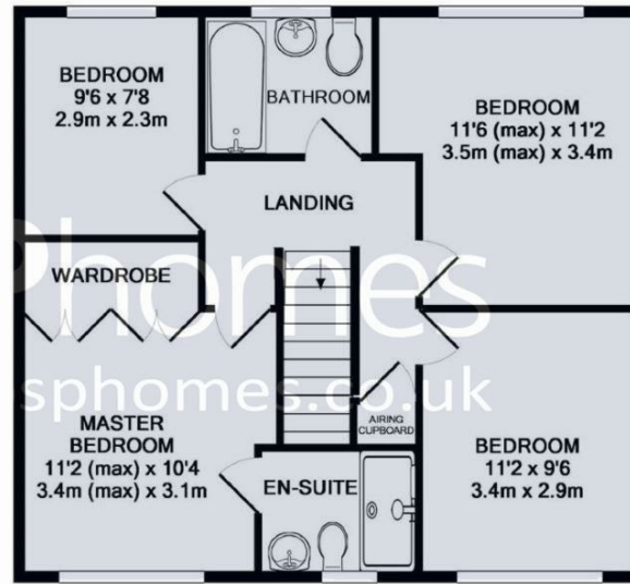
1ST FLOOR APPROX. FLOOR AREA 616 SQ.FT. (57.3 SQ.M.)
